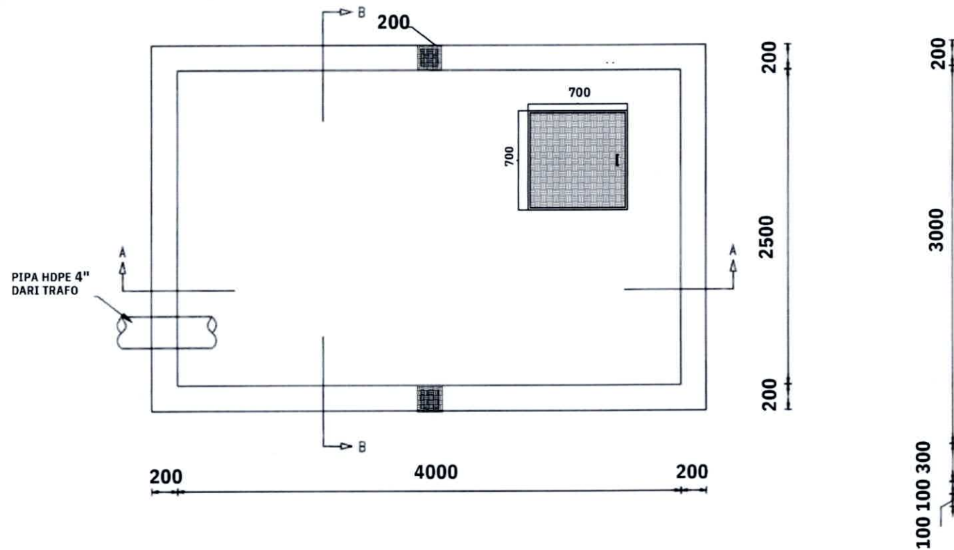
TOP VIEW
